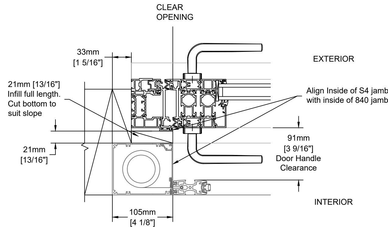
Horizontal Section Jamb with Handle
